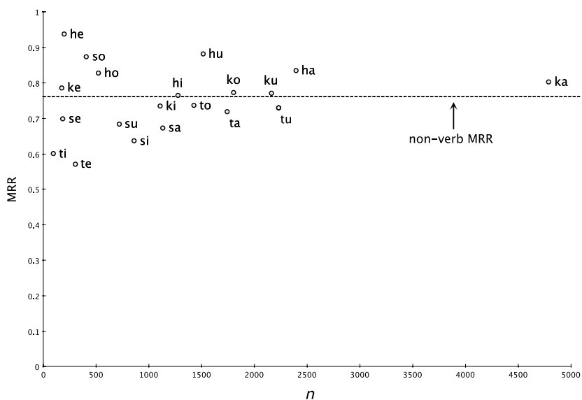
Figure 2 DATABASE Mean Rendaku Rates for non-verb E 2 -initial moras (data from Irwin & Miyashita 2013)
