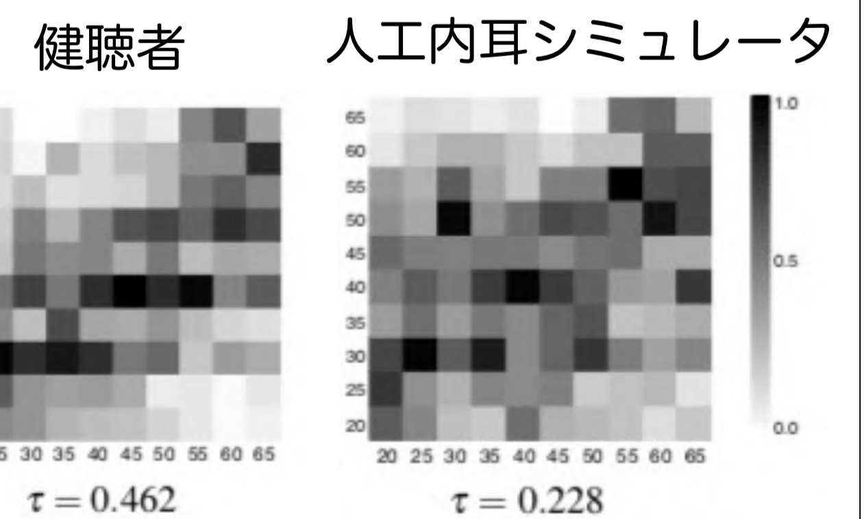
\tau = 0.462 \tau = 0.228
