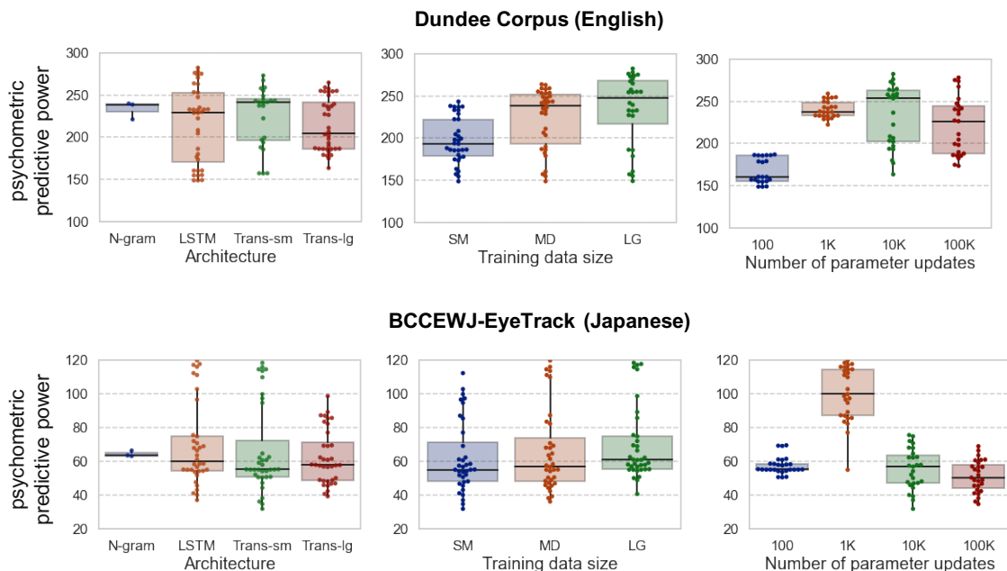
Figure 3: Separate effect of model architecture, training data size, and the number of parameter updates for LMs’ psychometric predictive power in each language. Each point corresponds to each LM. The box shows the quartiles of the data. The whiskers show 1.5 times interquartile range.
