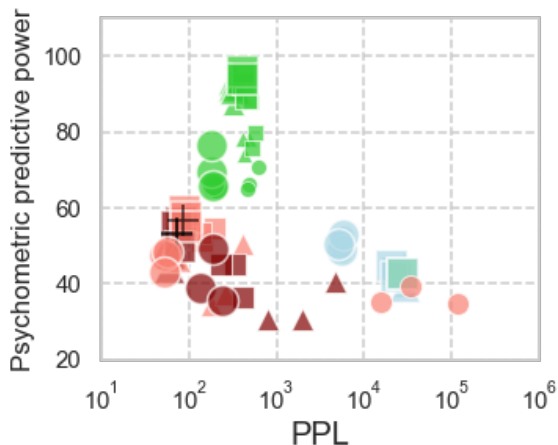
Figure 6: Relationship between PPL (X-axis) and psychometric predictive power (Y-axis). Each point corresponds to each LM. Low score on X-axis indicates the high linguistic accuracy of the model. High score on Y-axis indicates that the model has a high psychometric predictive power. Note that X-axis is on a log scale. The shape, color, and size of each point is same as Figure 2.
