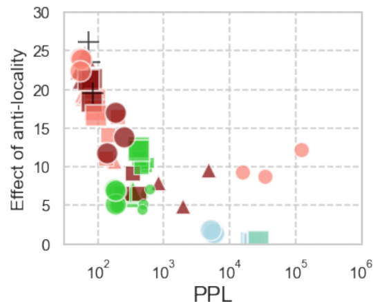
Figure 7: Relationship between PPL (X-axis) and the effect of the anti-locality (Y-axis). Each point corresponds to each LM. Low score on X-axis indicates the high linguistic accuracy of the model. High score on Y-axis indicates that the surprisals computed by the corresponding model are highly biased towards the anti-locality effect. Note that X-axis is on a log scale. The shape, color, and size of each point is same as Figure 2.
